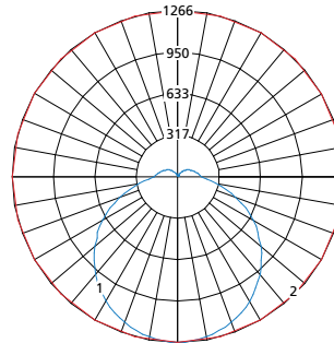
Model: H1212FM-PP-MW-50L40K-DV
