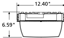
H1212FM
